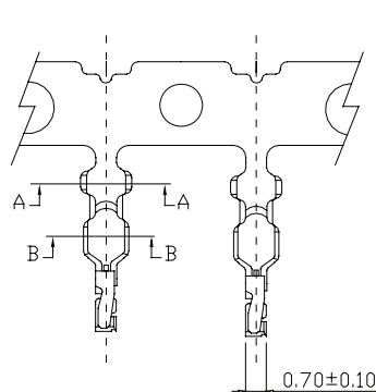
Part No.:1003H-T-L
